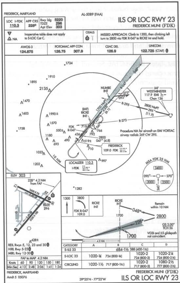
Figure 12. IFR Approach Chart—NOT FOR NAVIGATION
