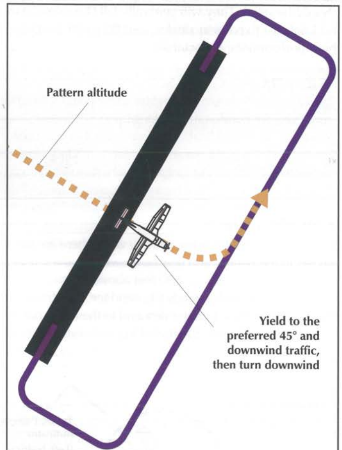
Figure 10. Alternate Midfield Entry from Upwind Leg Side of Airport
